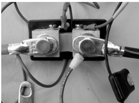
The shunt hook-up shows the use of heavy 4-gauge direct wiring and swaged lug terminals. Also, you need to add a proper-value fuse to protect the meter.
